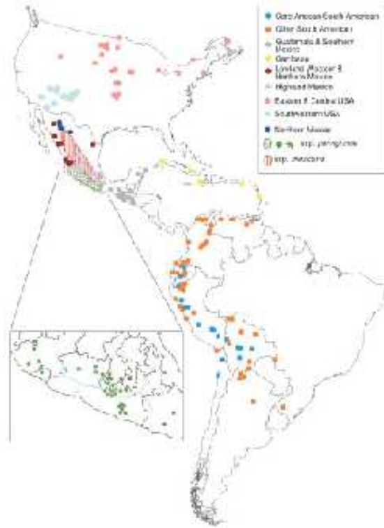
Fig. 1. Geographic distribution of maize landraces in the Americas. The distribution is based on the geographic origin of 1,200 maize landraces from 59 countries in the Americas (67). Color codes and southern Mexico (14), Caribbean (16), low and medium and northern Mesoamerica (15), Highland Mesoamerica (14), Central America (14), Caribbean (14), Mexico (14), northern Mexico (14), USA (14), and Mexico (14). Landraces are color-coded by geographic origin: Central America (blue), Caribbean (orange), Mexico (green), Central America (yellow), Yucatan (red), Mesoamerica (purple), Highland Mexico (brown), Mexico (grey), and USA (black). The inset map shows the geographic distribution of 1,200 maize landraces in the Yucatan region.
